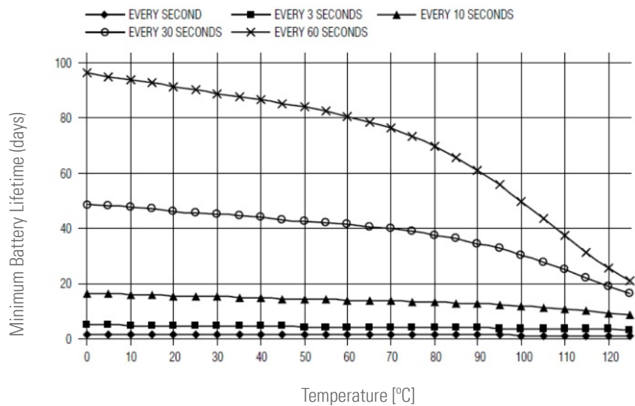
Battery Lifetime vs Temperature at fast sample rates (high resolution)
