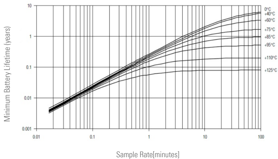
Battery Lifetime vs Different Sample Rates (high resolution)
