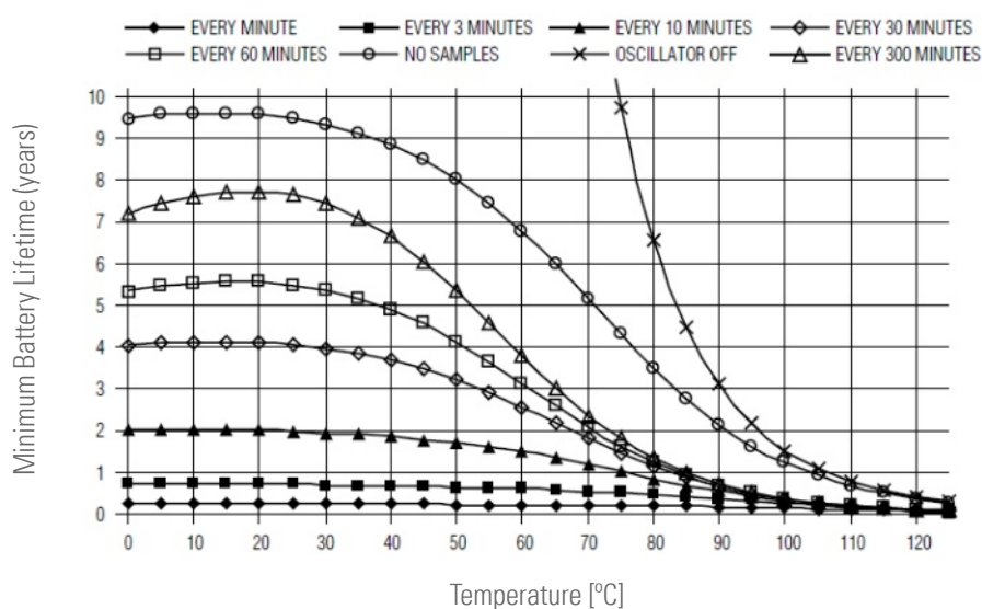
Battery Lifetime vs Temperature at slow sample rates (high resolution)
