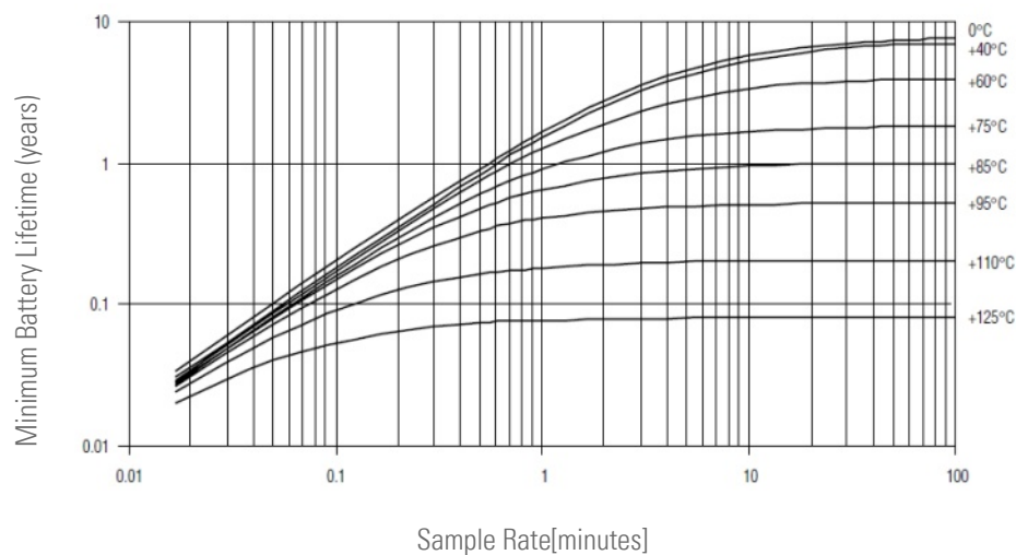
Battery Lifetime vs Different Sample Rates (standard resolution)
