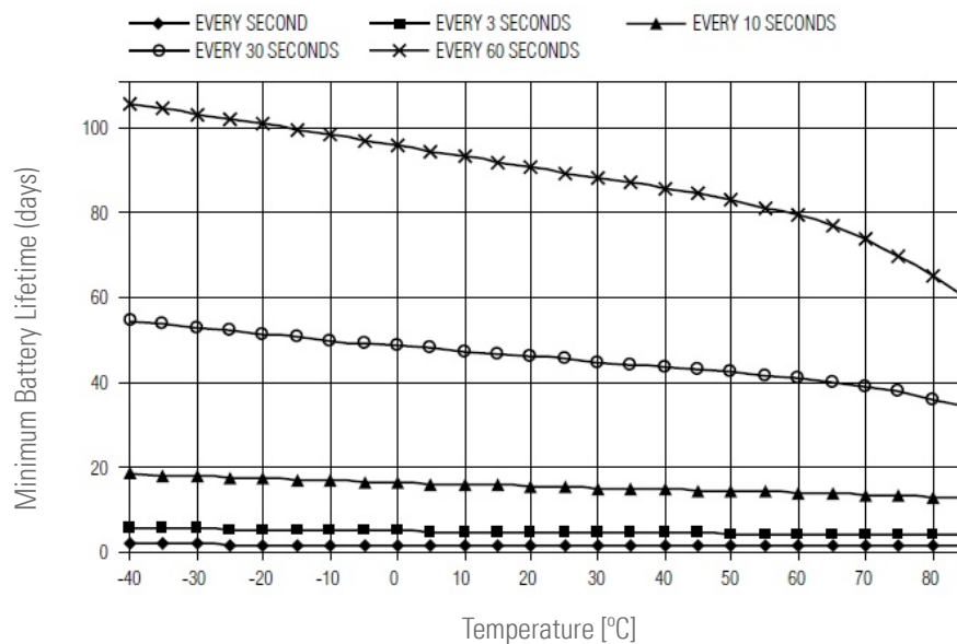
Battery Lifetime vs Temperature at fast sample rates (high resolution)
