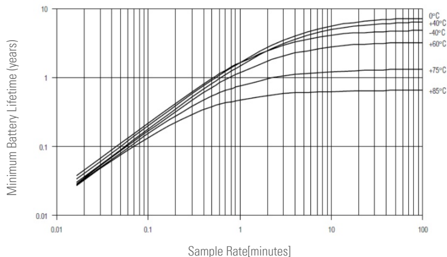
Battery Lifetime vs Different Sample Rates (standard resolution)
