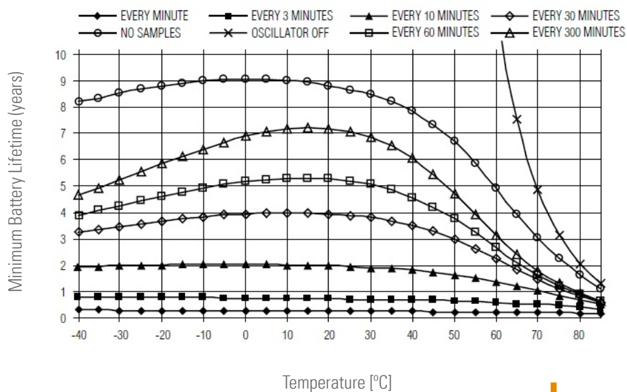
Battery Lifetime vs Temperature at slow sample rates (high resolution)
