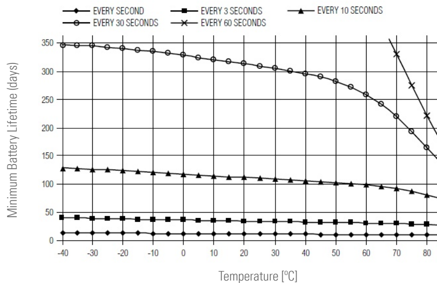
Battery Lifetime vs Temperature at fast sample rates (standard resolution)
