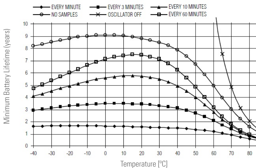
Battery Lifetime vs Temperature at slow sample rates (high resolution)
