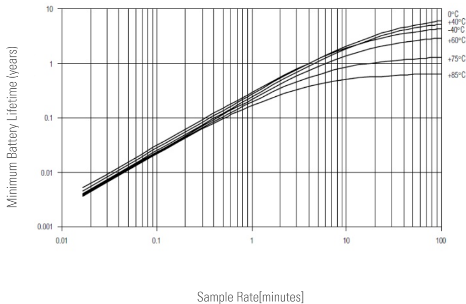
Battery Lifetime vs Different Sample Rates (high resolution)
